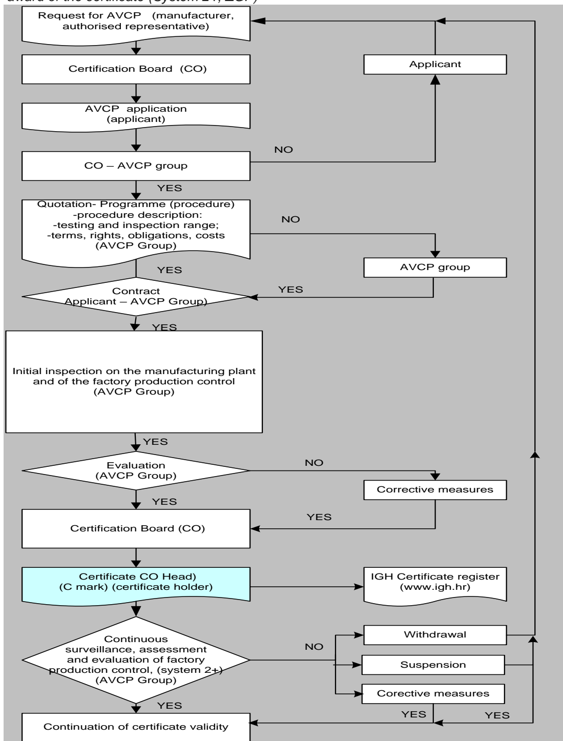
Flowchart - Procedure for the assessment and verification of the constancy of performance and the award of the certificate (System 2+, ZGP)
